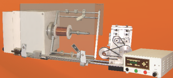
Spiral Winding Machine with programmable pitch for continuous winding on fiber / wire or tube along with pay off and take-up system
