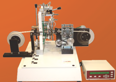
Continuous Winder on flexible strip with programmable pitch
