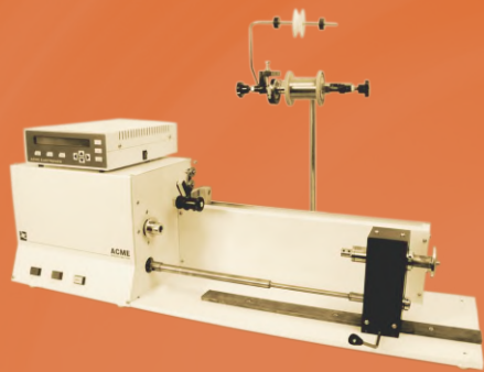
Long Axial Winder for winding length upto 24 inch long with driven tail stock
